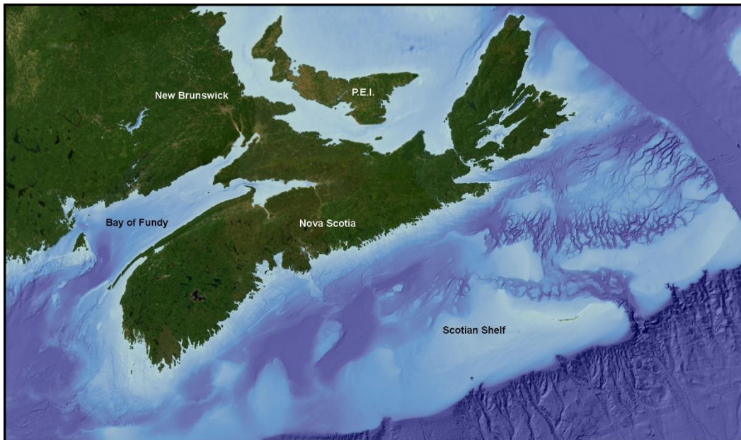
Illustration of the study area including a part of the Scotian Shelf
